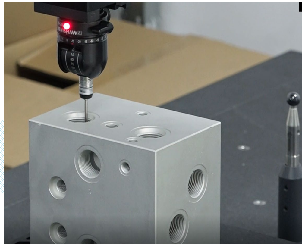
CMM measure
