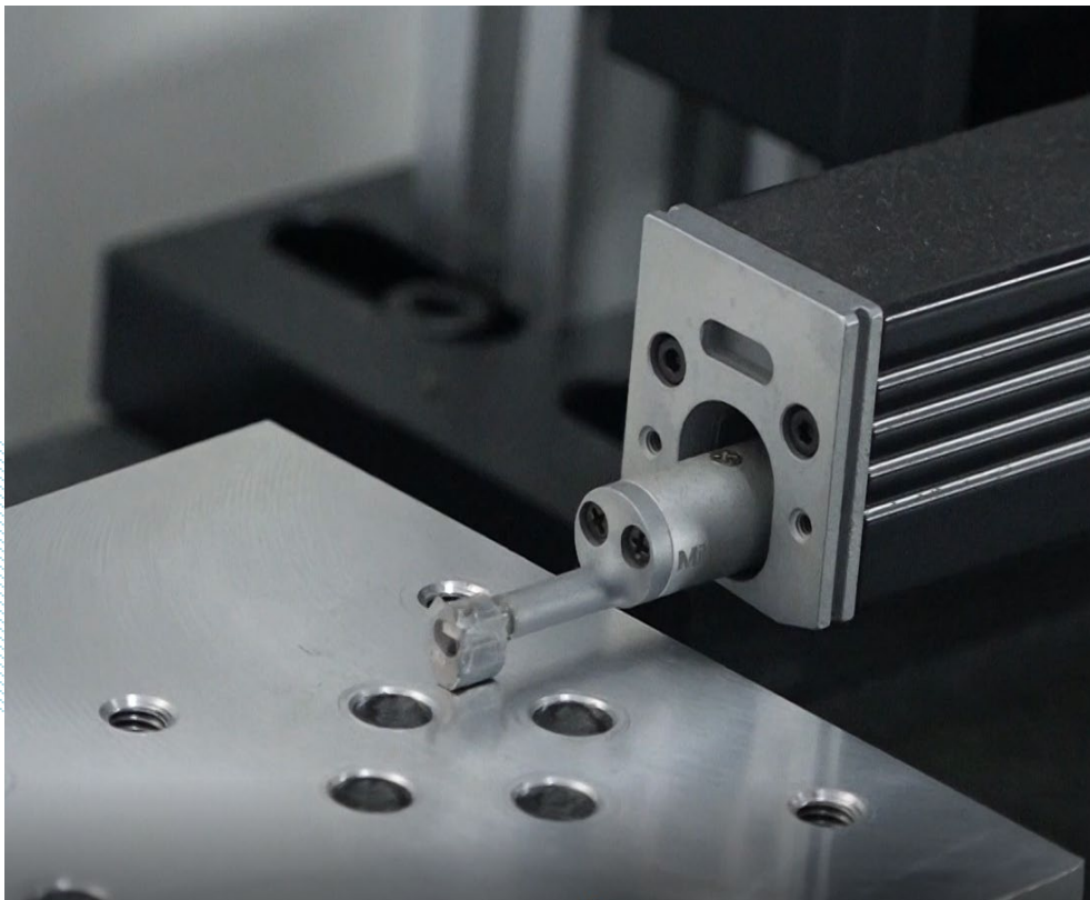
Checking surface roughness
