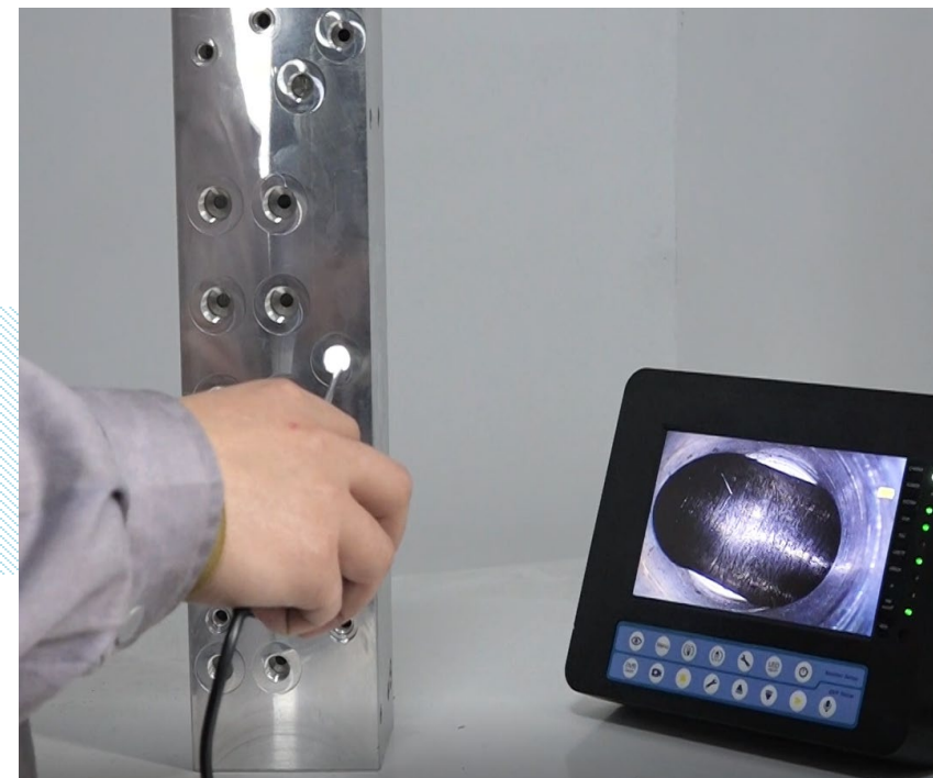
Burs checking with endoscope
